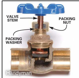
Gate Valve
